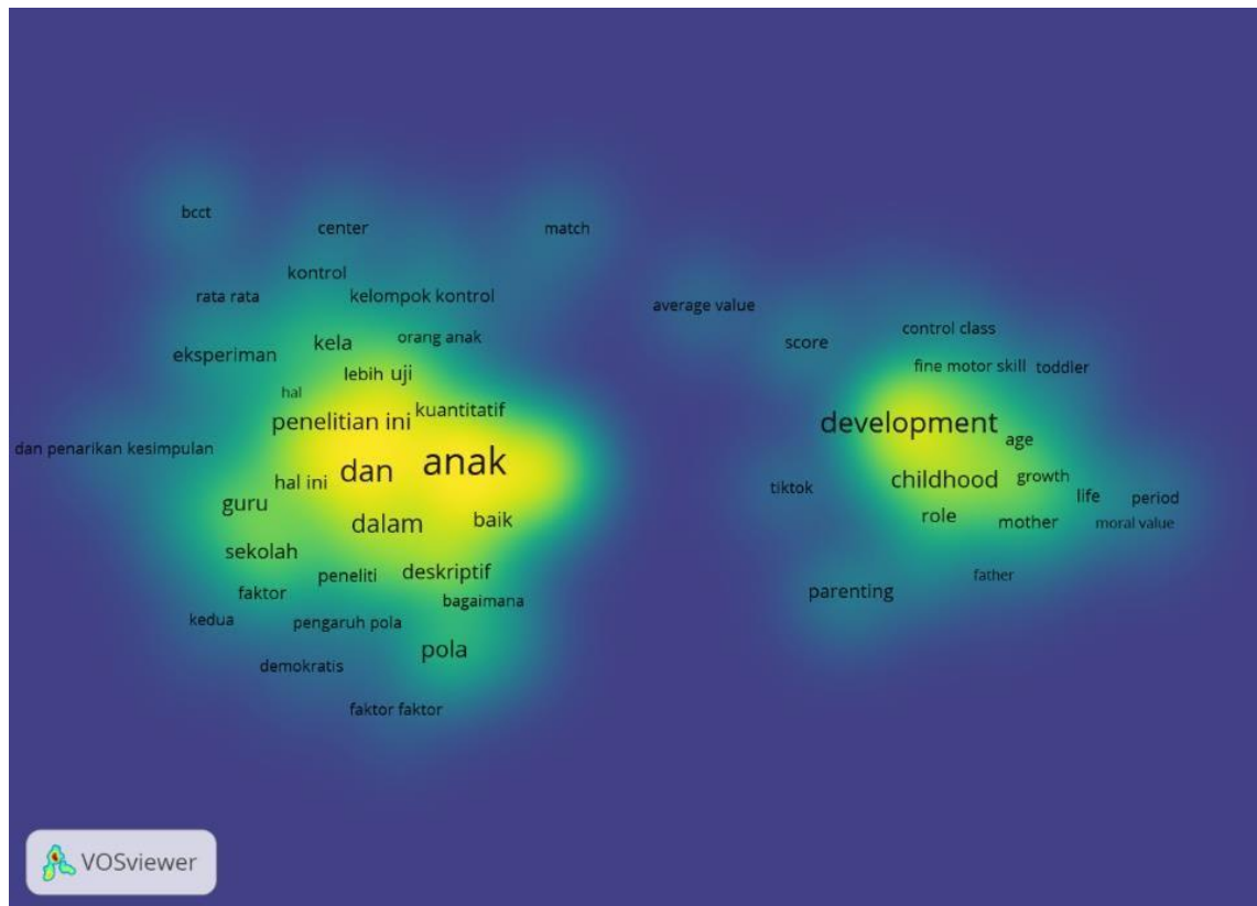
Gambar 5. Density Visualization
